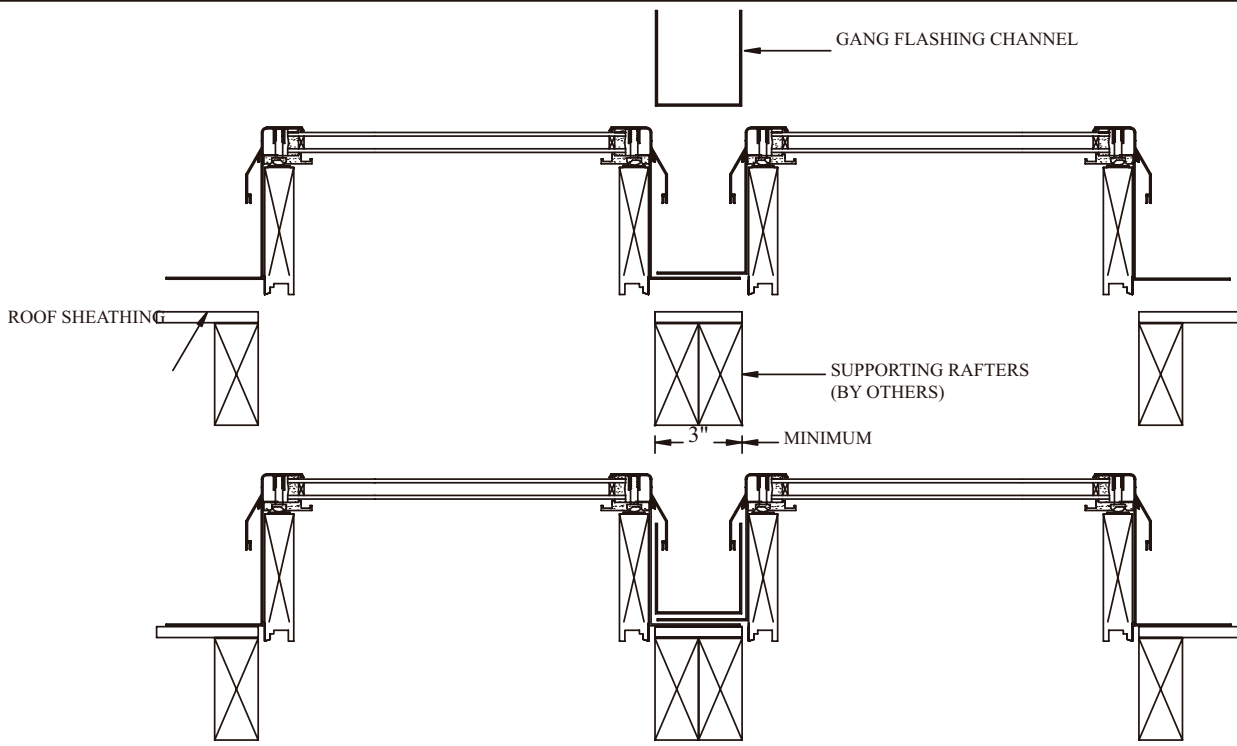
STANDARD STARLIGHT SKYLIGHTS
