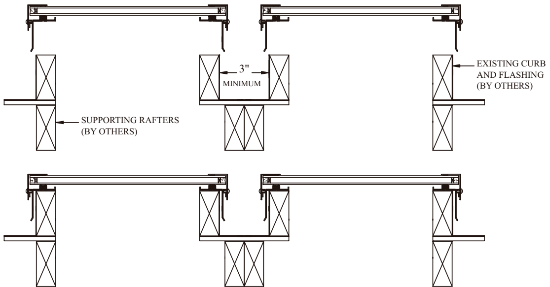
STANDARD CURB MOUNTS
