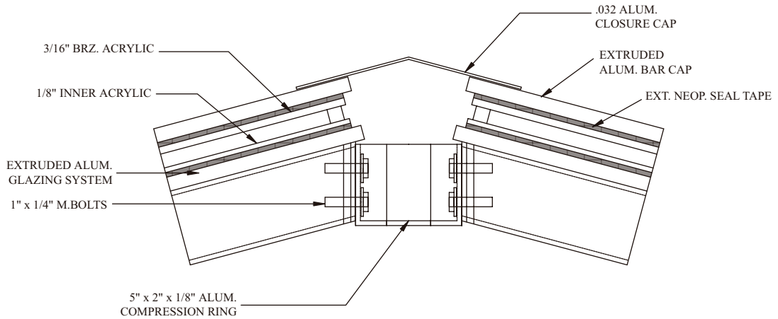
COMPRESSION RING DETAIL
